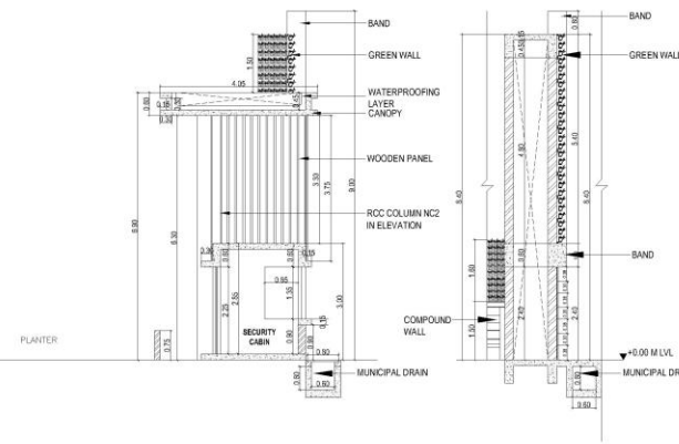
SECTION CC'
