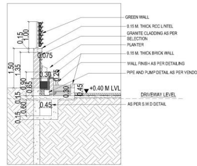
DETAIL OF WATER BODY- SECTION CC'
