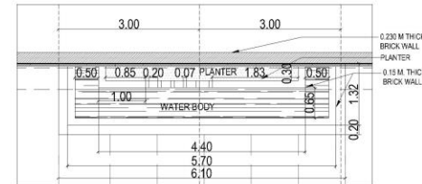
DETAIL A- PLAN OF WATER BODY
