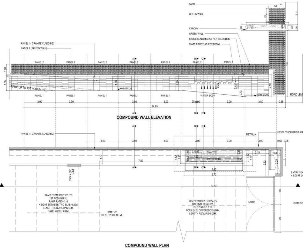
COMPOUND WALL PLAN
