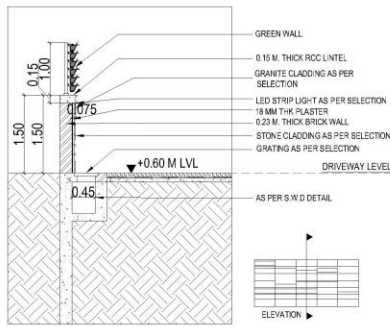
DETAIL OF PANEL 1 (STONE CLADDING) SECTION AA'
