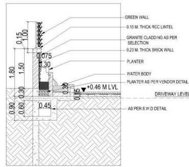
DETAIL OF WATER BODY- SECTION BB'
