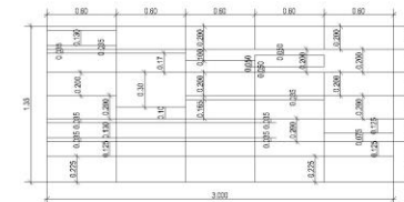
DETAIL OF PANEL 1 (STONE CLADDING)
